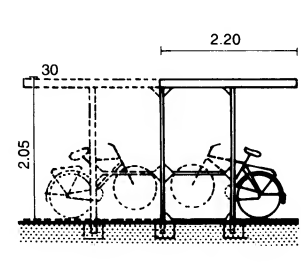
⑯ Cycle sheds
